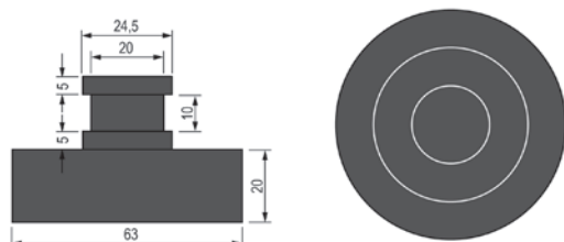
Pressring
