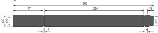
Pressring
